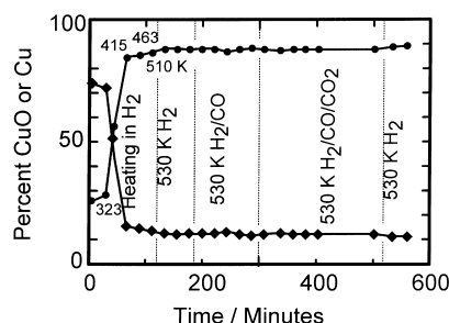
Fig. 7. Fractions of Cu-containing phases identified by analysis of Cu K-near-edge spectra. (●) Cu metal; (◆) CuO-like phase. Conditions were 0.42 MPa, heating rate 2° min -1 .
